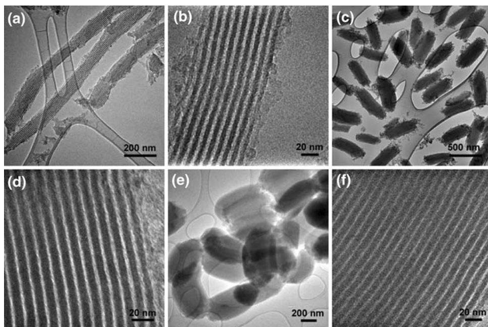
Fig. 3 TEM and HRTEM images of extracted PMO nanostructures; a and b NFs, c and d NRs, e and f NEs
