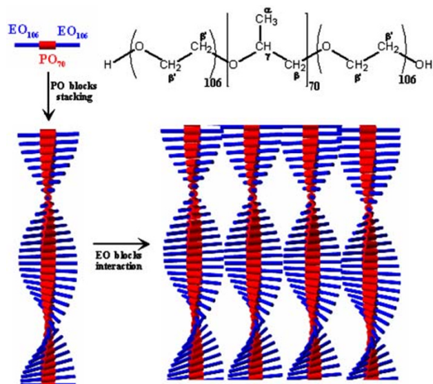
Scheme 1. Self-organization of stack-up \text{EO}_{106}\text{PO}_{70}\text{EO}_{106} into polymeric supramolecules
