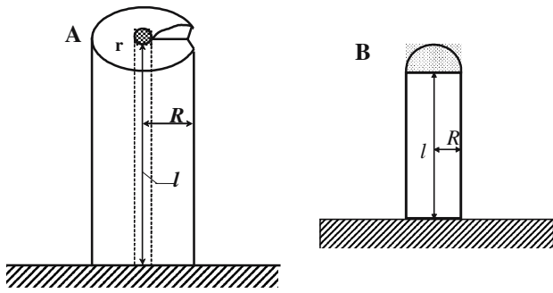
Fig. 1 Models of growing nanowhiskers: Fig.1A—growing nanotube. The length is l , the inner radius of the pipe is r ; the radius of the nanotube is R . The growth is secured by a screw dislocation. Fig.1B—growing nanowires by VLS mechanism
