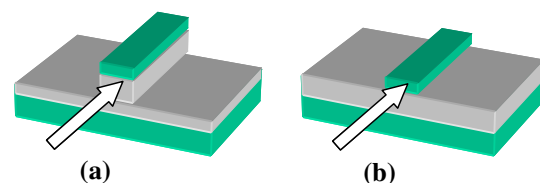
Fig. 6 (a) A high-index-contrast and (b) deep-etched waveguide built on SOI wafer, light enters in direction of arrow. The waveguide may be further buried under a cladding layer
