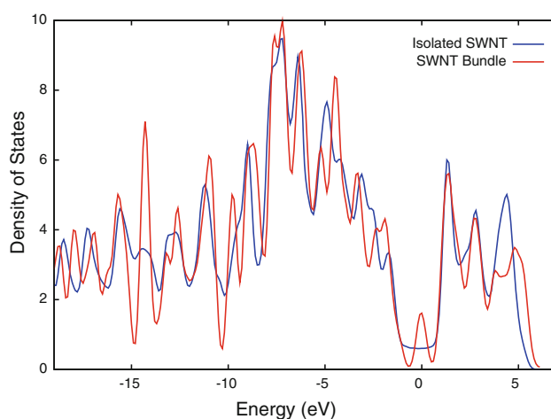
Fig. 3 Density of states comparison of a (5,5) isolated SWNT vs. a (5,5) SWNT bundle. Note the enhanced density of states at the Fermi level. The Fermi levels of both plots are centered on 0 eV. This increased density of states will yield a higher quantum capacitance per unit volume for a bundle when compared to its constituent individual tube
