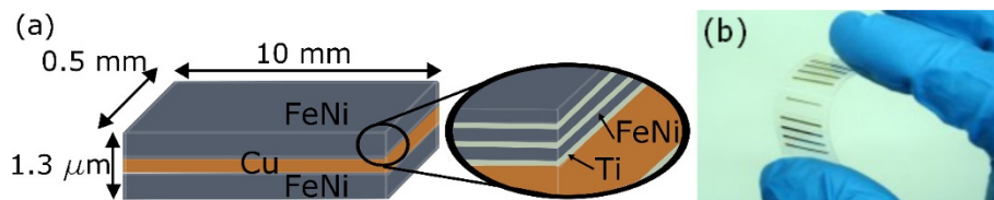
Figure 1 Scheme of the GMI structure and the samples deposited onto a COC substrate. (a) Scheme of the [\text{FeNi}(170 \text{ nm})/\text{Ti}(6 \text{ nm})]_3/\text{Cu} (250 nm)/ [\text{Ti}(6 \text{ nm})/\text{FeNi}(170 \text{ nm})]_3 GMI structure used in this study. (b) Samples deposited onto a COC flexible substrate.
