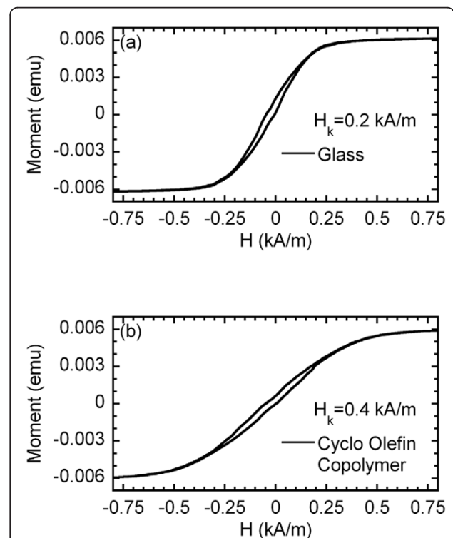
Figure 2 M(H) curves. (a) Sample deposited onto the rigid glass substrate and (b) onto the flexible substrate.
