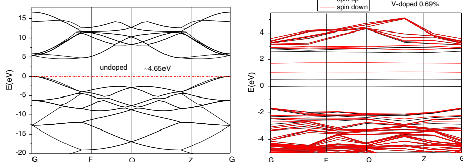
Figure 1 The band structures of undoped and V-doped diamonds.
