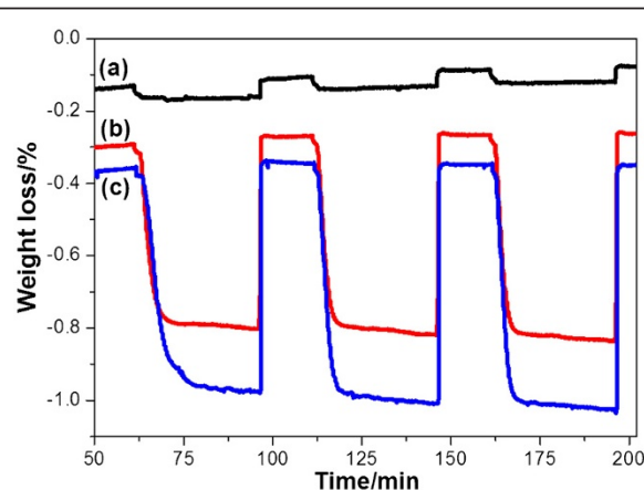
Figure 4 TG profiles of calcined samples ( 1,000^\circ\text{C} , 20 h) at 600^\circ\text{C} , which show oxygen release/storage properties. (a) \text{CeO}_2 , (b) \text{Ce}_{0.5}\text{Zr}_{0.5}\text{O}_2 , and (c) \text{Ce}_{0.5}\text{Zr}_{0.3}\text{Al}_{0.2}\text{O}_{1.9} .
