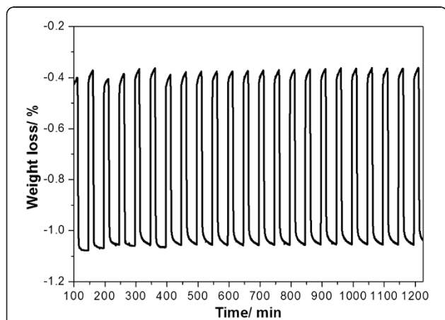
Figure 5 TG profiles during measurement of OSC at 600°C for Ce 0.5 Zr 0.3 Al 0.2 O 1.9 (1,000°C, 20 h) after 22 cycles. The profiles show oxygen release/storage properties.
