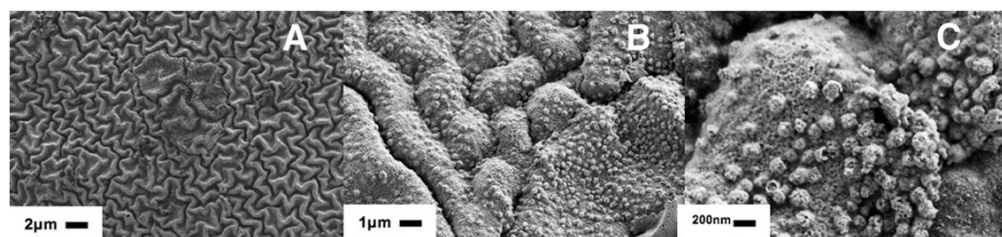
Figure 3 High-resolution SEM images of the surface of Purolite C100E modified with Ag-NPs. Magnification A < B < C . (A) High-resolution SEM image of the increase of cross-linking degree of Purolite C100E resin modified with Ag-MNPs (B,C).
