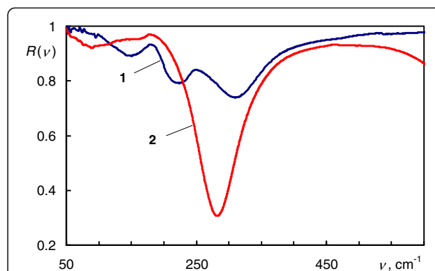
Figure 2 Experimental reflectance spectra of \text{Ge}_2\text{Sb}_2\text{Te}_5 . 1 - amorphous, 2 - crystalline.
